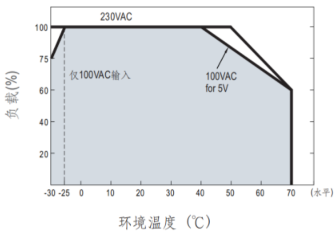
降额曲线:
